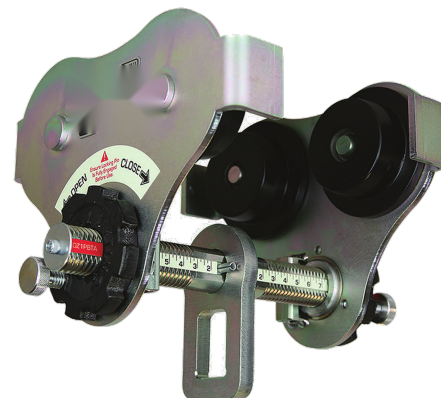
PUSH BEAM TROLLEY MODELS OZ05PBTA – OZ3PBTA
